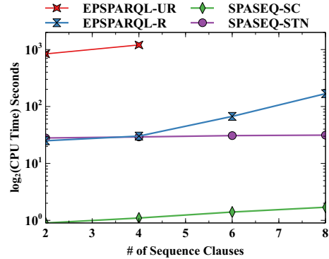
Figure 17. Comparison of SPASEQ (Strict Contiguity (SC) and Skip-Till-Next (STN)) with EP-SPARQL (Recent (R) and Unrestricted (UR)) by increasing the number of sequence clause for SMD dataset and queries over a window of 40 minutes.
