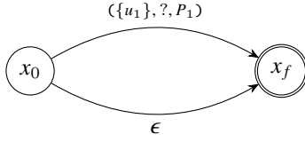
Figure 24. Compilation of the Optional Operator for ((u_1, P_1)?)
