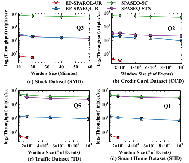
Figure 16. Average Throughput comparison (triples/second) of SPASEQ (Strict Contiguity (SC) and Skip-Till-Next (STN)) with EP-SPARQL (Recent (R) and Unrestricted (UR)) over the four selected datasets (SMD, CCD, TD and SHD).
