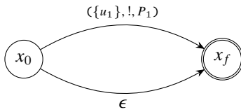
Figure 25. Compilation of the Negation Operator for ((u_1, P_1)!)
