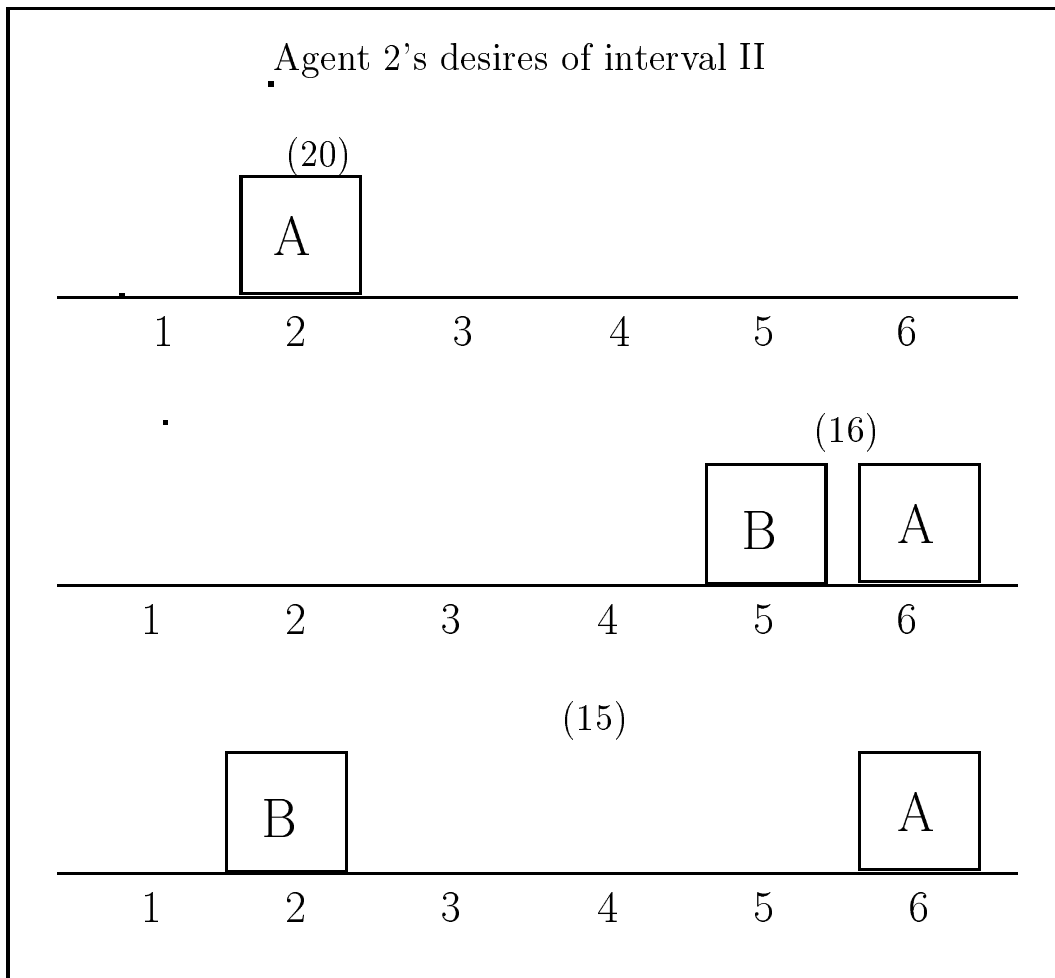
Fig. 6. The desired world states for Agent 2, interval II.
