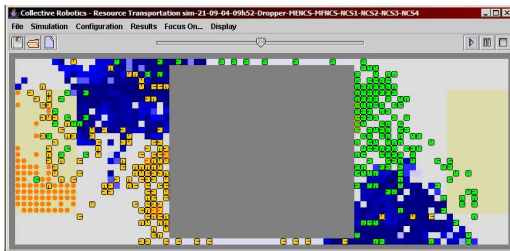
Figure 2: Incoming robots for the top corridor for two different behaviors: unblocking behavior (left) and anticipative unblocking behavior (right).
